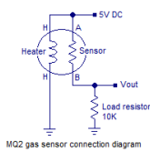
MQ2 gas sensor connection diagram
